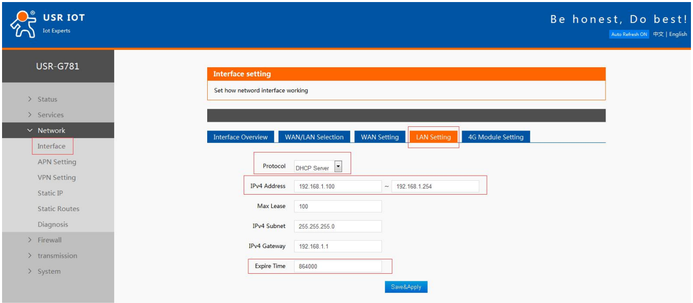
Figure 21 DHCP Server function configuration
